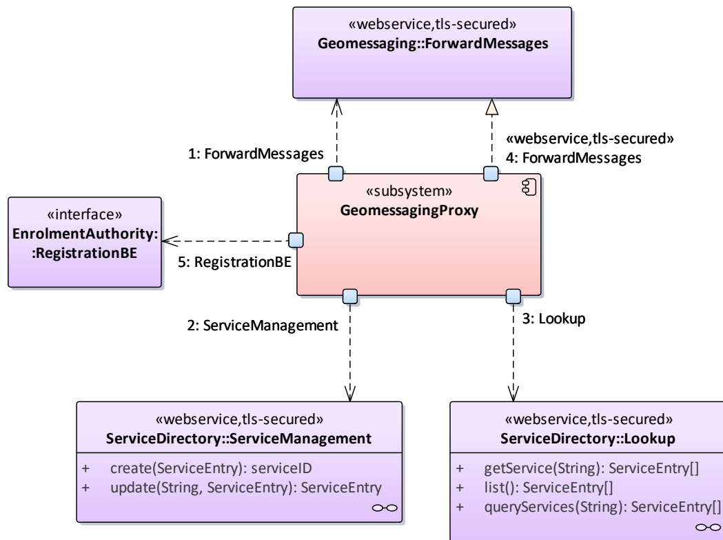
Figure 60: GeomessagingProxy
