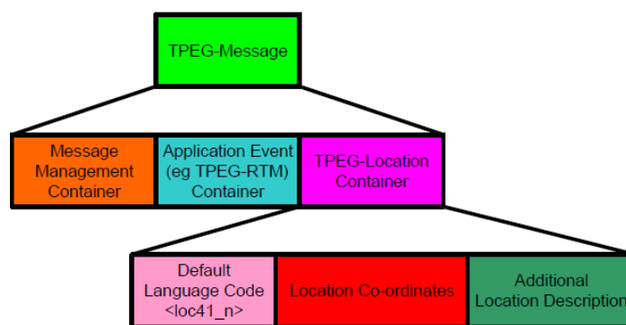
Figure 27: Principle structure of a TPEG message [5] (p.15)
