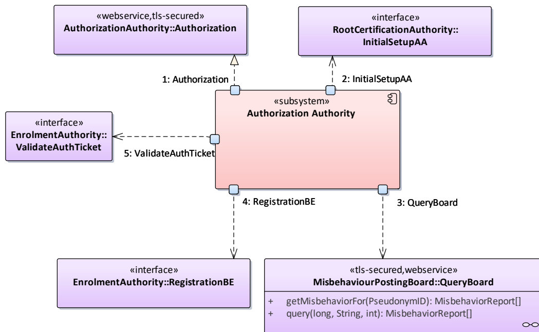
Figure 58: Authorization Authority
