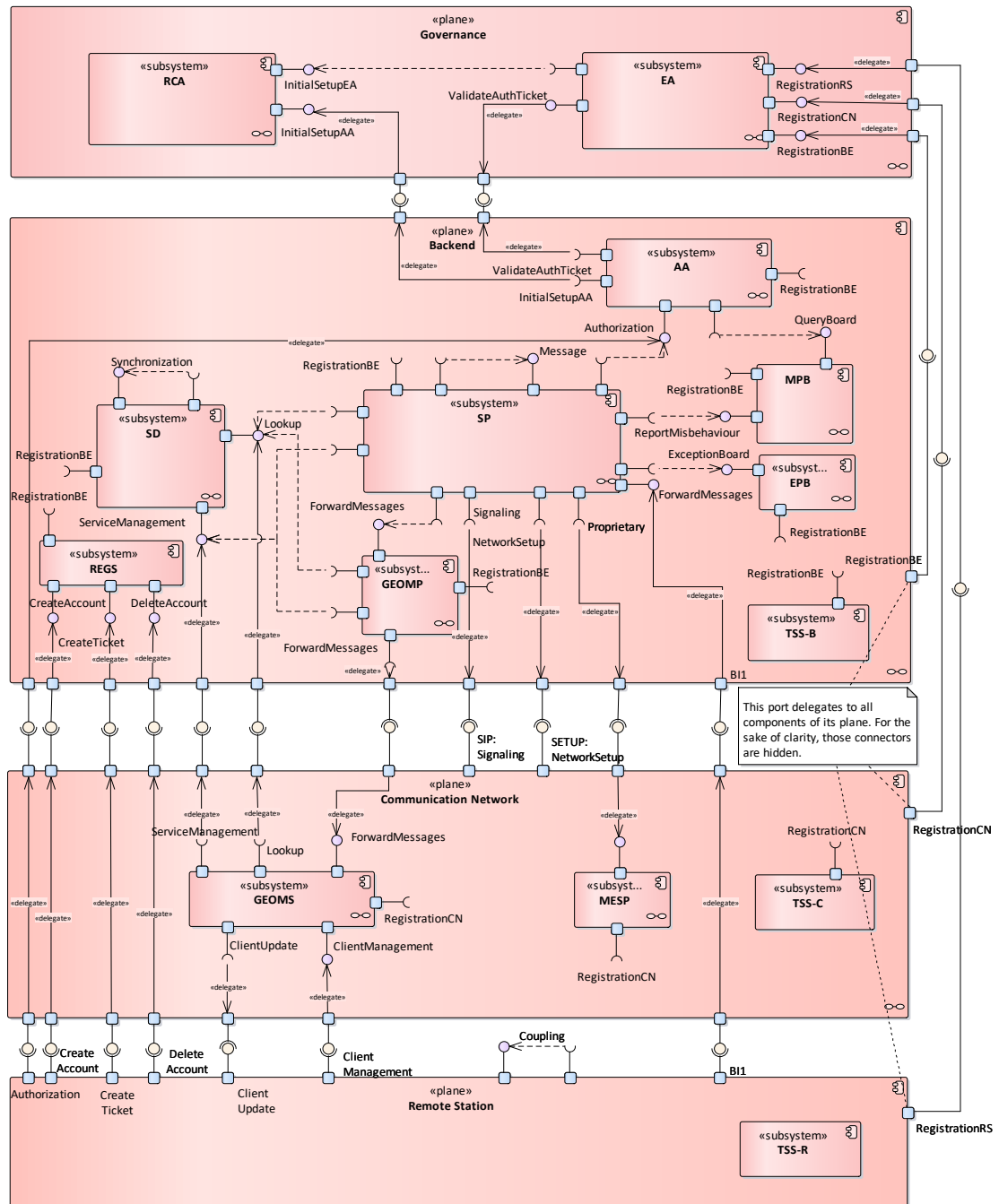
Figure 54: iKoPA high-level architecture
