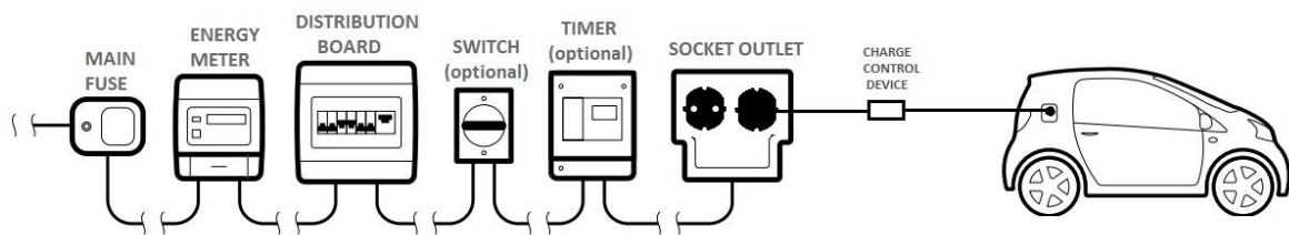
Figure 50: Typical Mode 2 charging connection [15]
