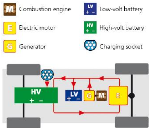
Figure 38: Common EV drive technology 15
