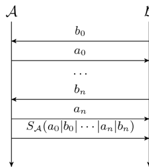
Figure 35: A basic distance bounding protocol
