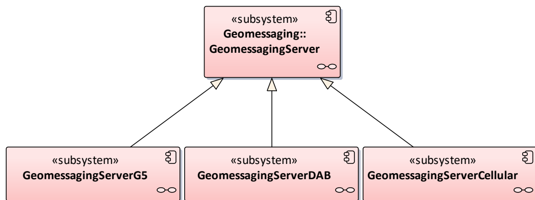
Figure 70: Geomessaging-Entities
