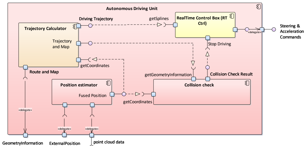
Figure 87: Autonomous Driving Unit
