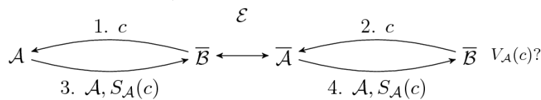
Figure 34: A relay attack on a challenge response authentication
