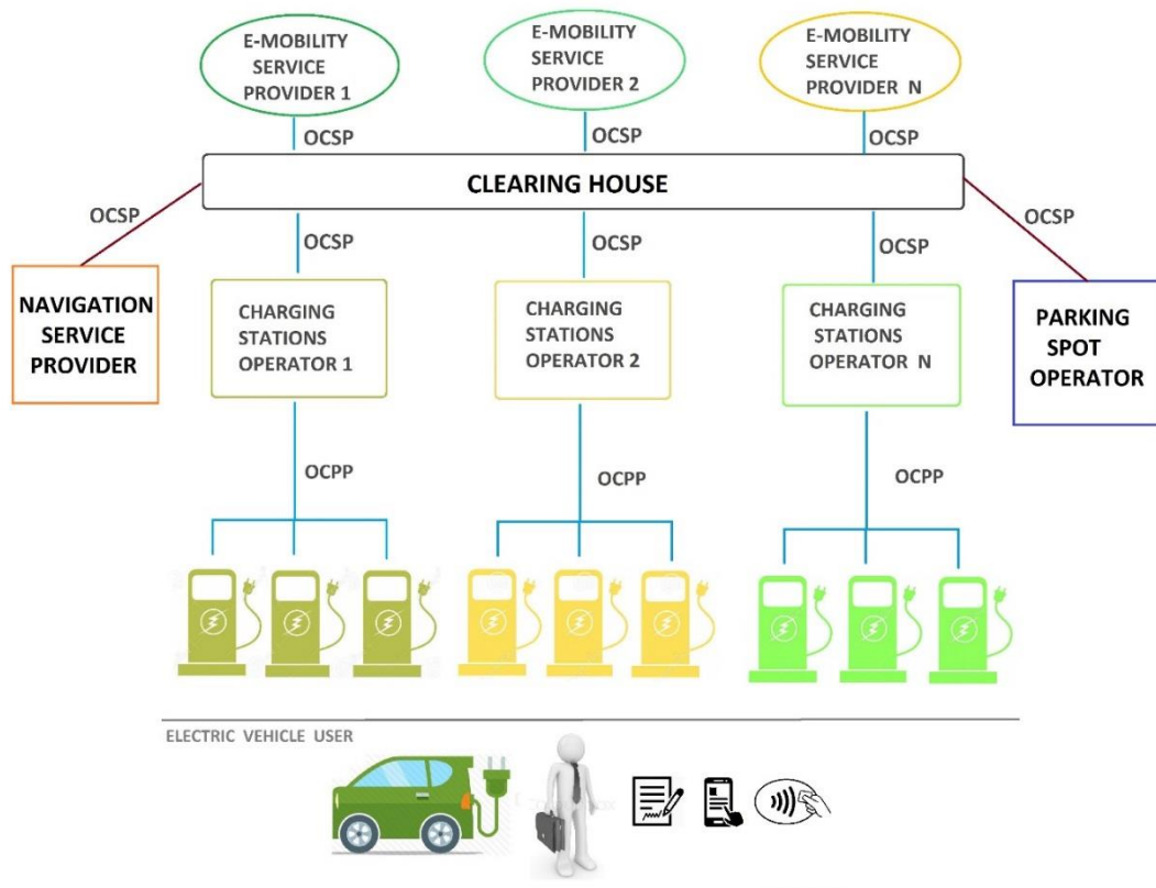
Figure 47: Charging actors
