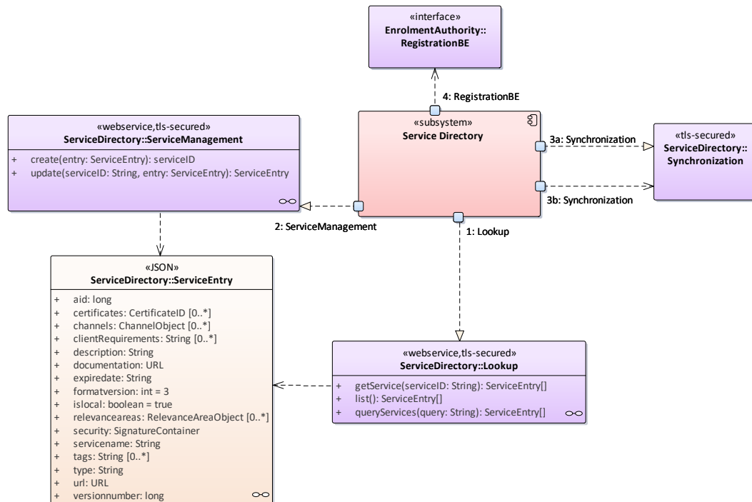
Figure 64: Service Directory
