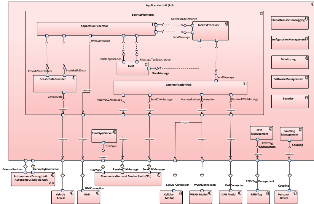
Figure 86: V-ITS-Station
