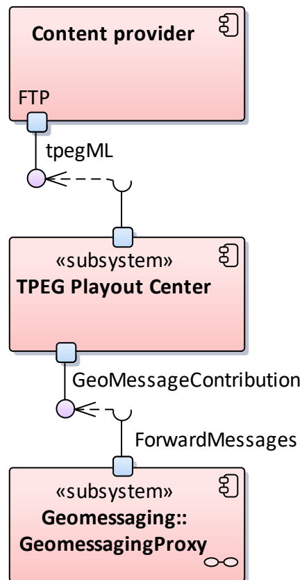
Figure 85: Traffic Message Distribution TPEG
