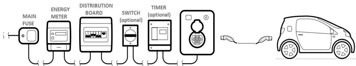
Figure 51: Typical Mode 3 charging connection [15]
