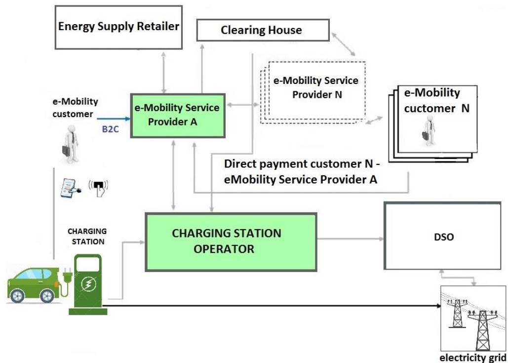
Figure 46: The independent e-mobility market model [11]
