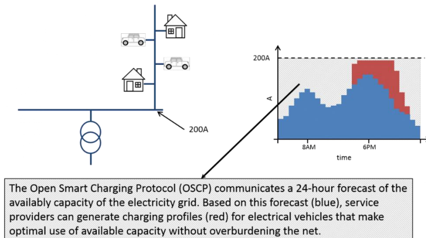
Figure 49: OSCP principle [14]
