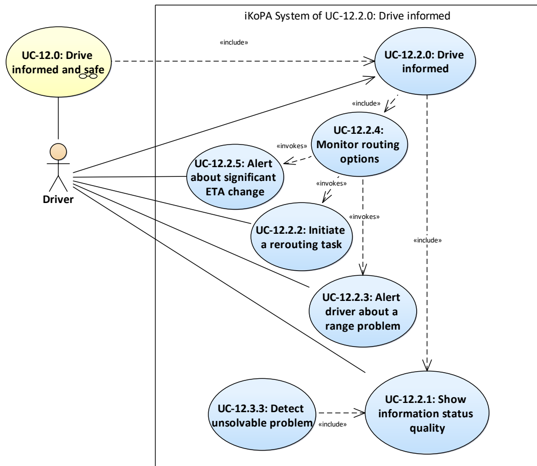
Figure 19: UC-12.2: Drive informed
