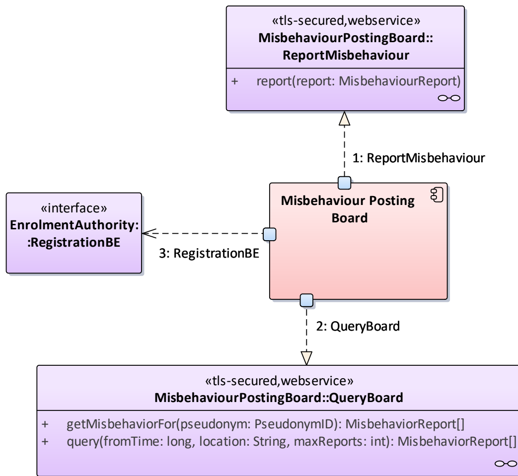
Figure 61: Misbehavior Posting Board
