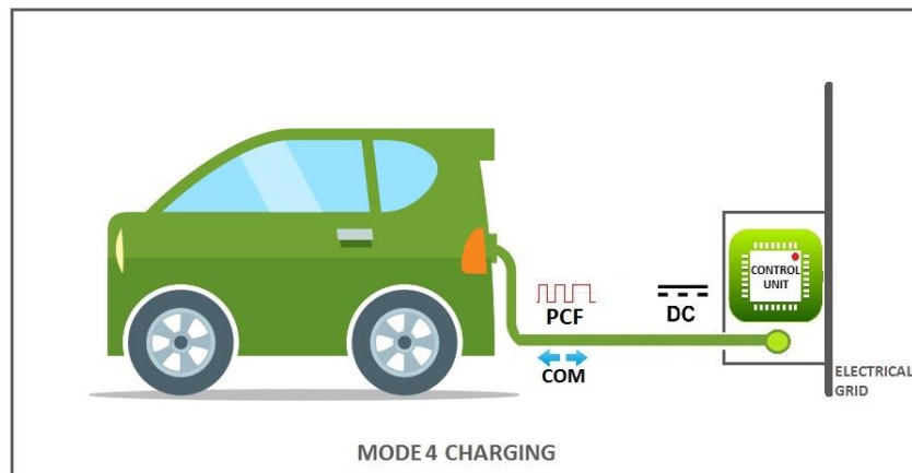
Figure 43: Mode 4 charging
