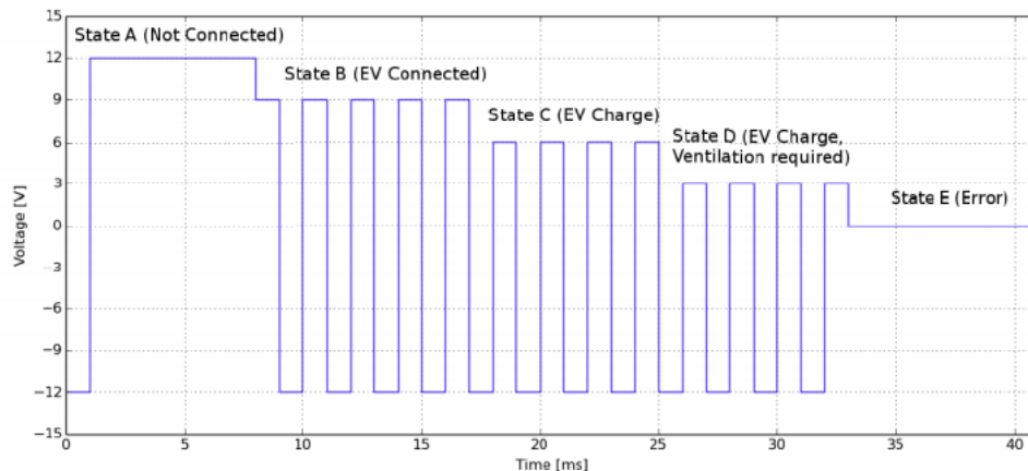
Figure 44: PWM signaling for Pilot control function [21]
