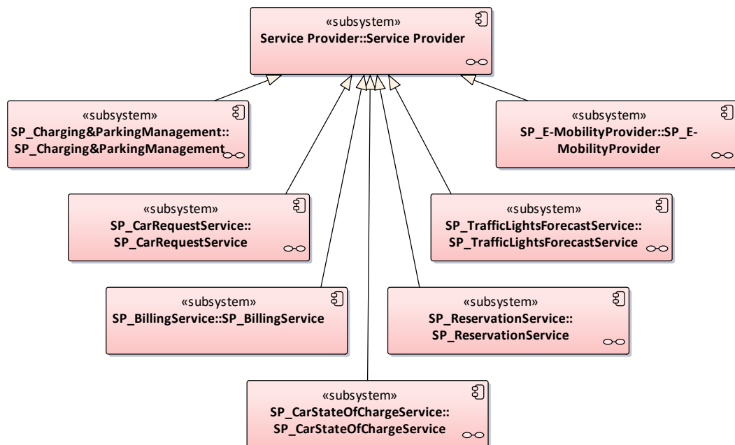
Figure 76: SP Overview
