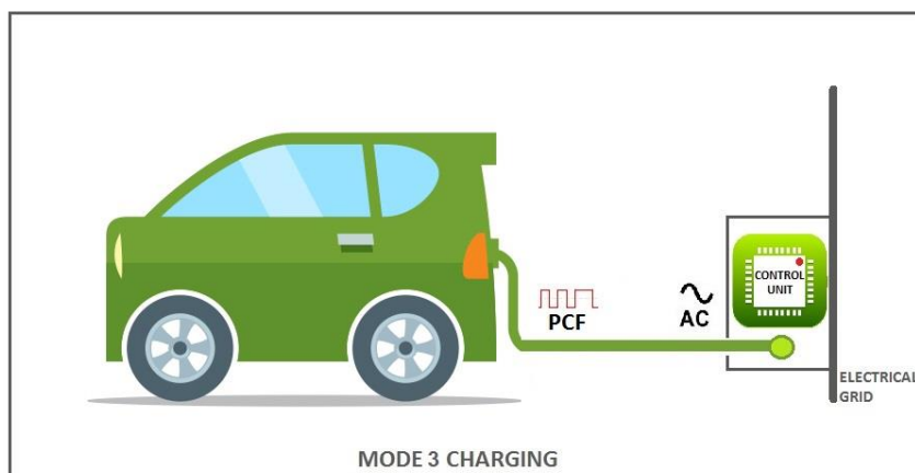
Figure 42: Mode 3 charging
