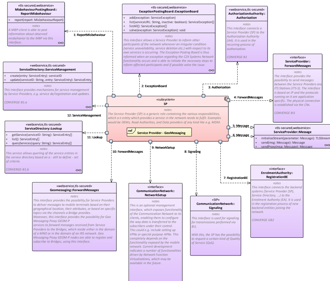
Figure 65: Service Provider
