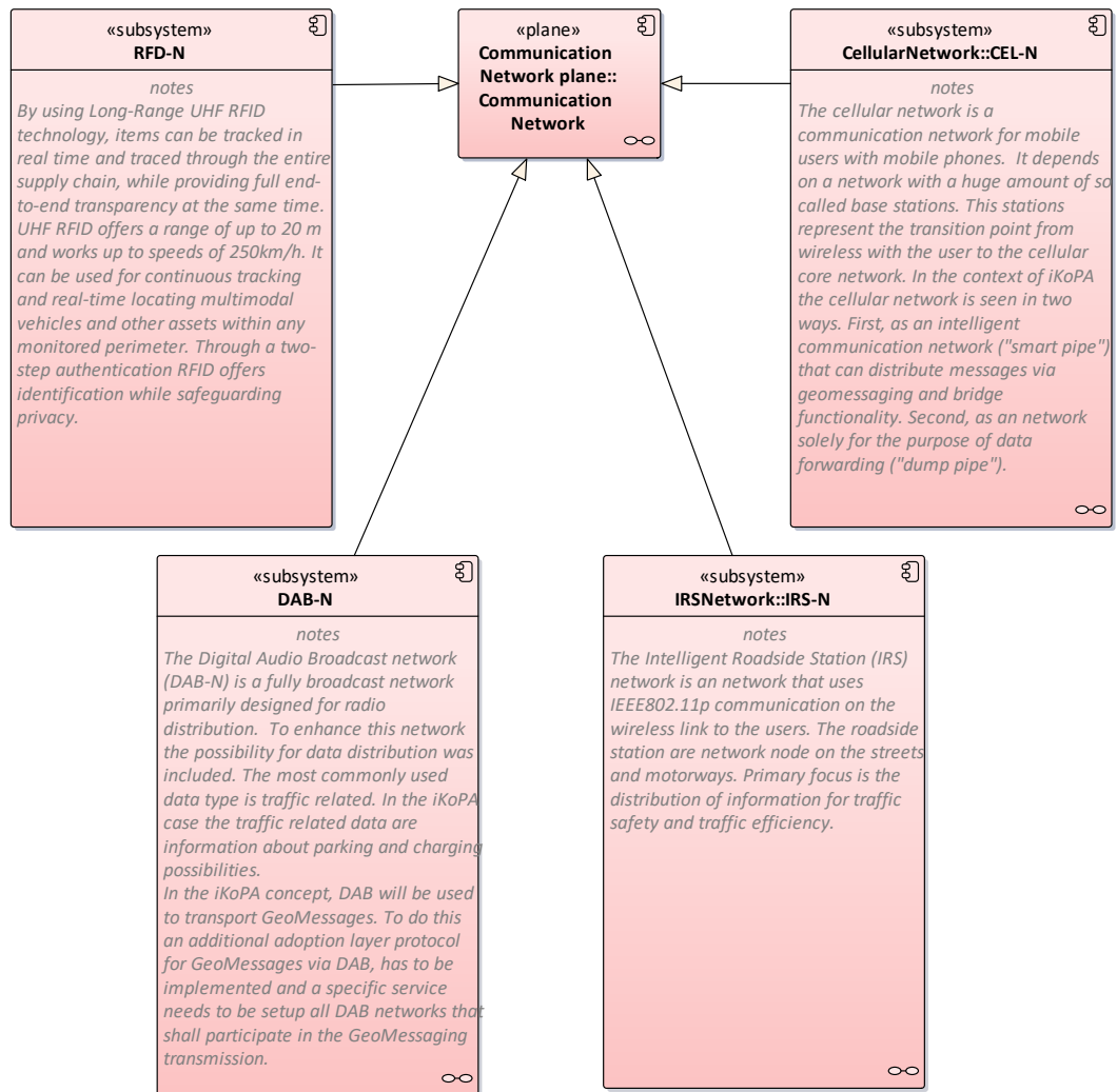
Figure 66: ComNet-Entities
