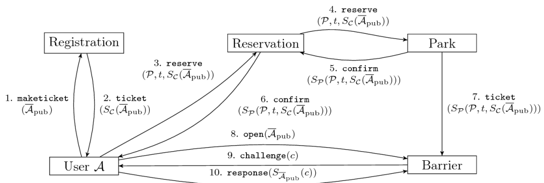
Figure 36: Message sequence reservation process
