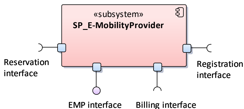
Figure 80: SP_E-MobilityProvider
