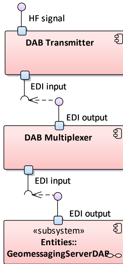
Figure 84: Traffic Message Distribution - DAB
