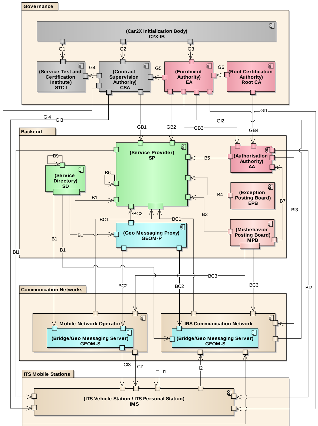
Figure 22: Overview on Car2X Systems Network Architecture [1]
