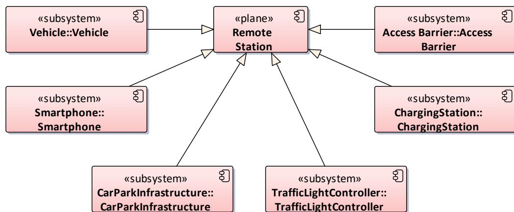
Figure 72: Remote Station
