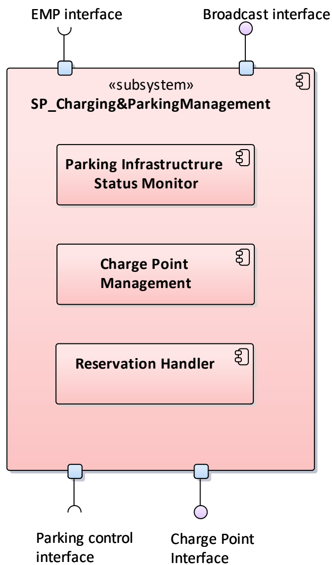
Figure 79: SP_Charge&ParkManagementService internal overview
