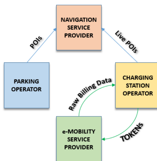
Figure 48: OCHP interfaces [13]
