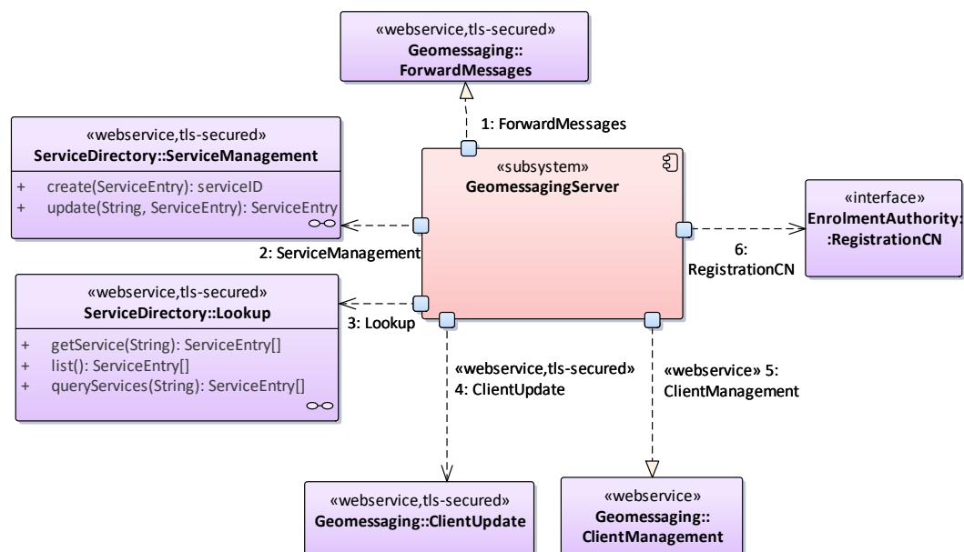
Figure 71: GeomessagingServer
