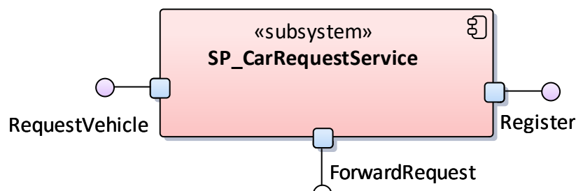
Figure 77: SP_CarRequestService
