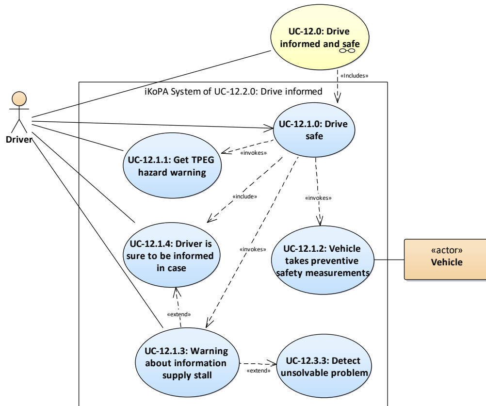
Figure 18: UC-12.1.0: Drive safe
