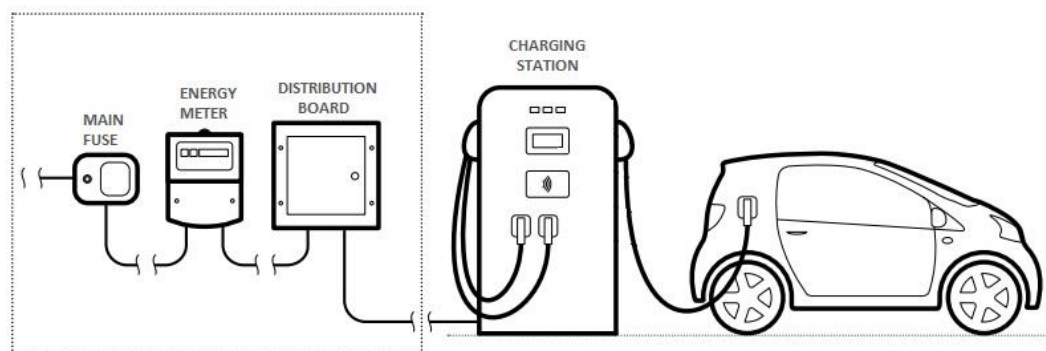
Figure 52: Typical Mode 4 charging connection [15]
